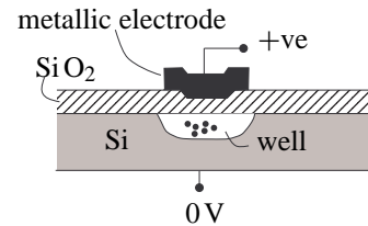
Figure 4: Charge collection beneath a semiconductor gate.
