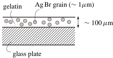
Figure 1: Photographic plate.
