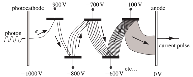
Figure 2: Photomultiplier tube.
